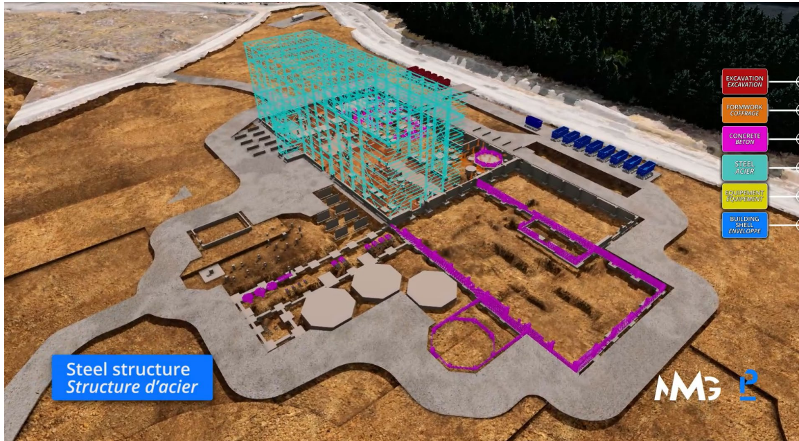
4D model of the Matawinie Mine construction timeline produced by Pomerleau using the BIM platform, available for viewing at https://youtu.be/rNvqCVHRzEw .
